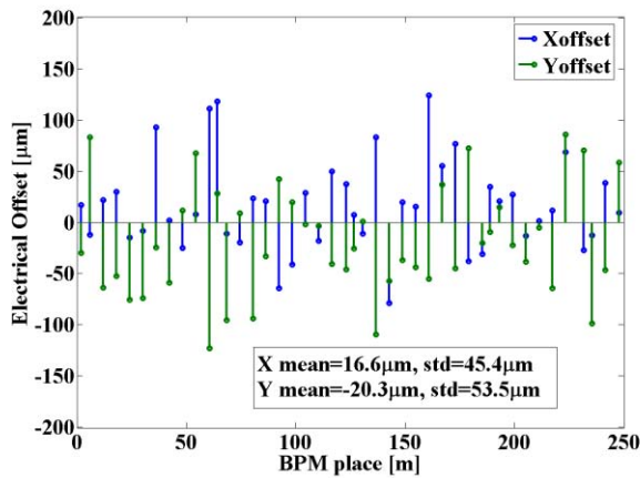
Figure 5: Electrical offset distribution for ALBA Booster BPMs.
