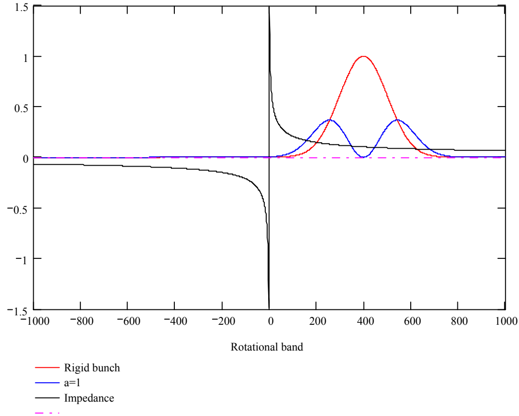
Power spectra and impedances, Bunch-length=10 cm
