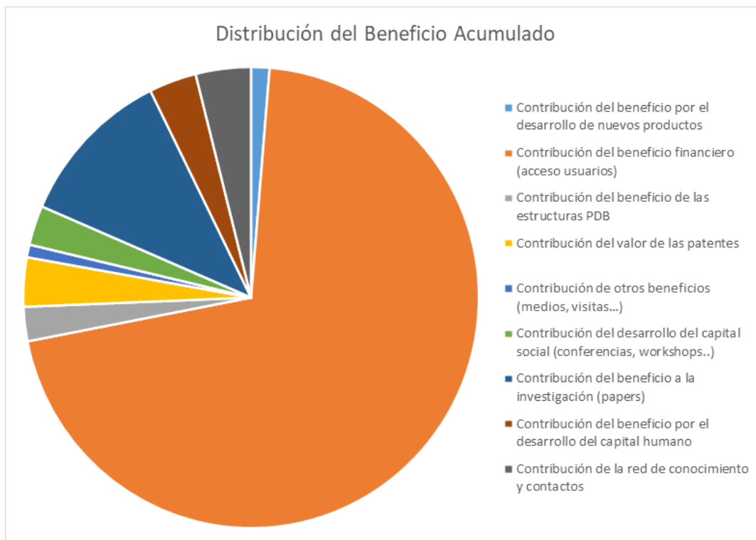
Figure 2.- Distribution of the cumulative net present value of ALBA II's benefit
