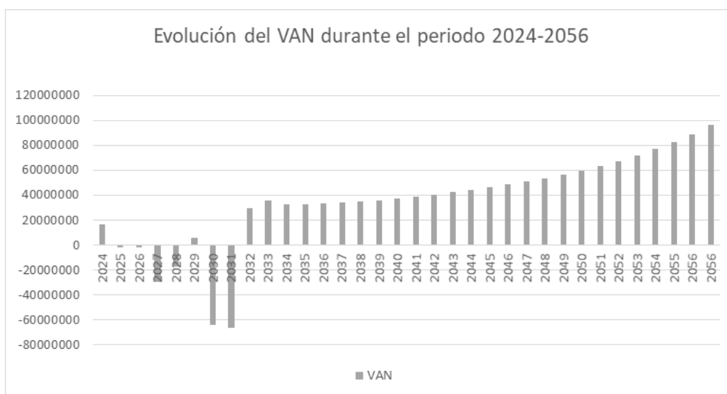
Figure 3.- Distribution of the net present value
